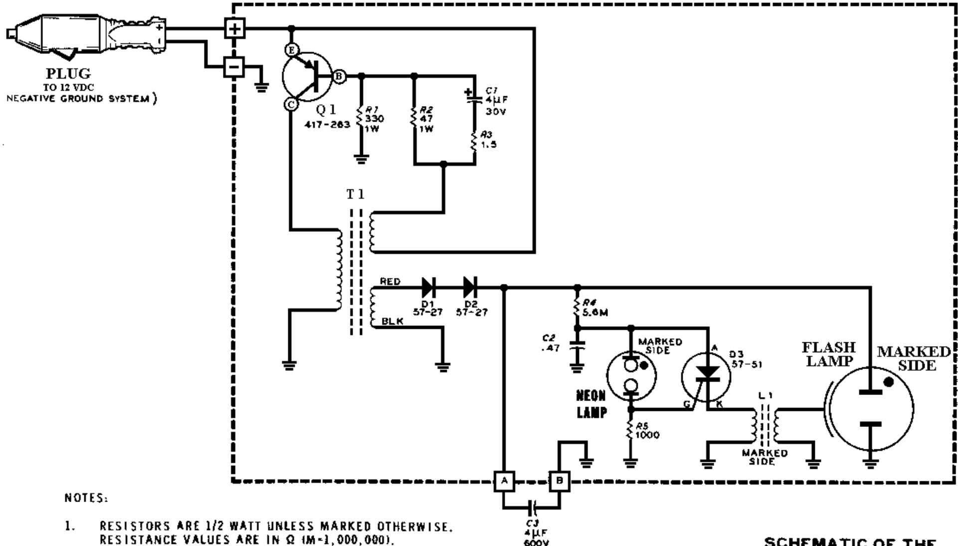
SCHEMATIC OF THE HEATHKIT® MODEL GD-1026 EMERGENCY STROBE LIGHT
