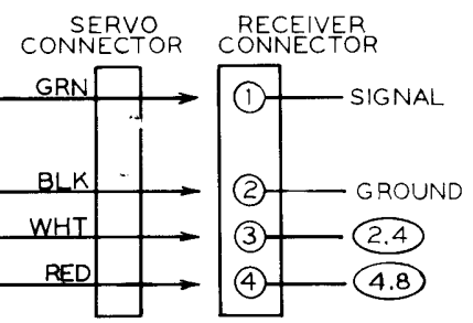
SCHEMATIC OF THE HEATHKIT® SUBMINIATURE DIGITAL PROPORTIONAL SERVO MODEL GDA-19-42
