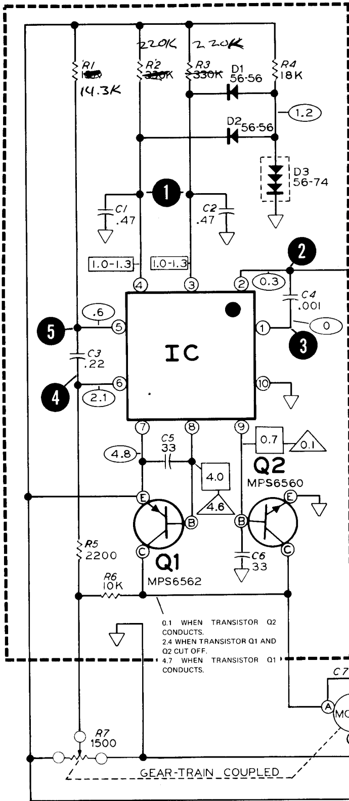
SCHEMATIC OF THE HEATHKIT® SUBMINIATURE DIGITAL PROPORTIONAL SERVO MODEL GDA-19-42
