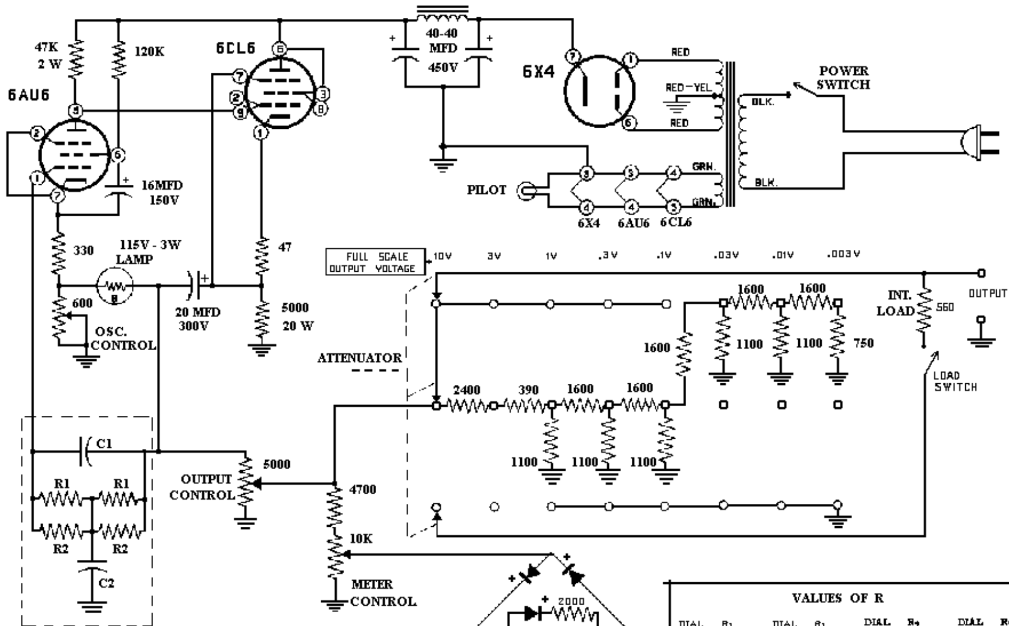
SCHEMATIC OF THE HEATHKIT® AUDIO GENERATOR MODEL IG-72
