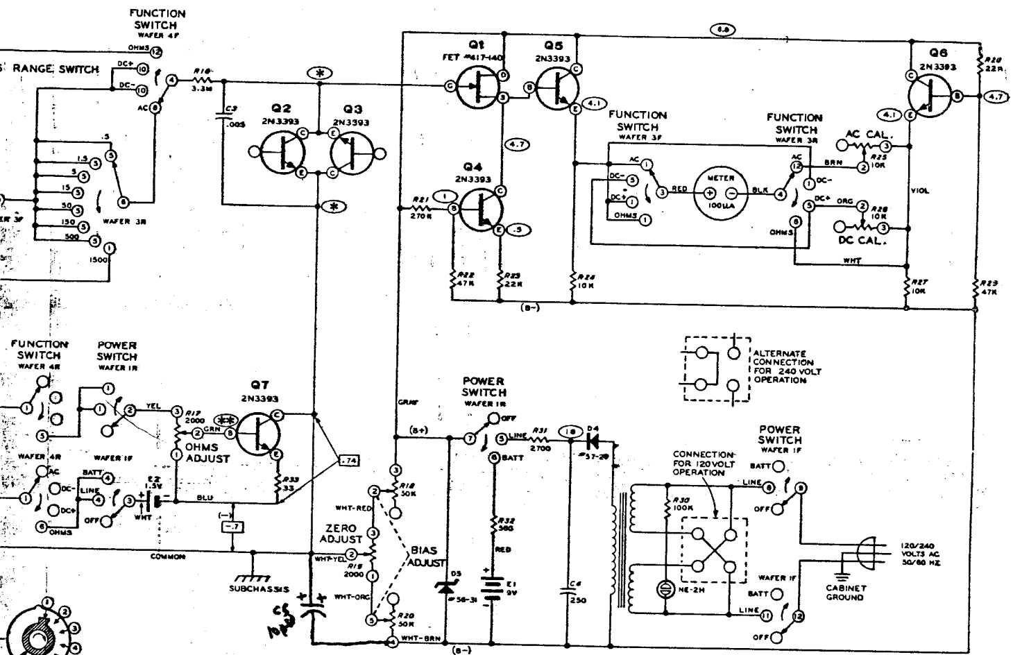
SCHEMATIC OF THE HEATHKIT® SOLID-STATE VOLTMETER MODEL IM-16
