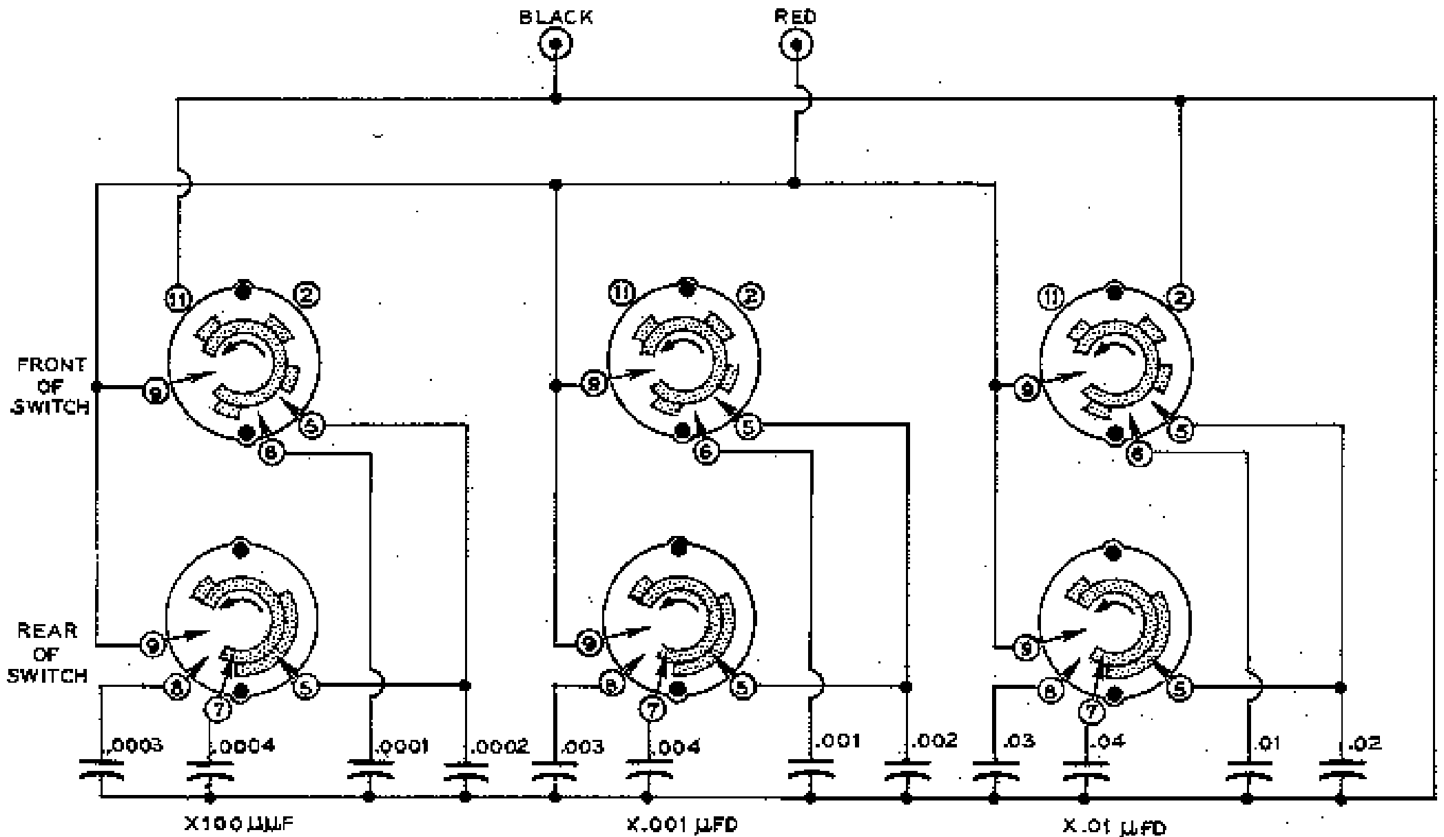
SWITCHES ARE VIEWED FROM REAR AND FULLY COUNTERCLOCKWISE SCHEMATIC DIAGRAM MODEL IN-21
