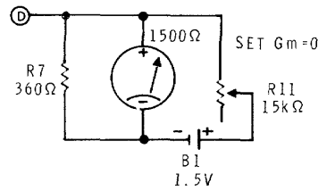
Gm=0 Figure 12
