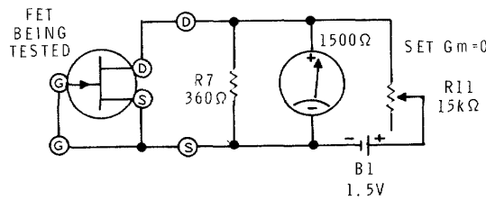
Gm Figure 13
