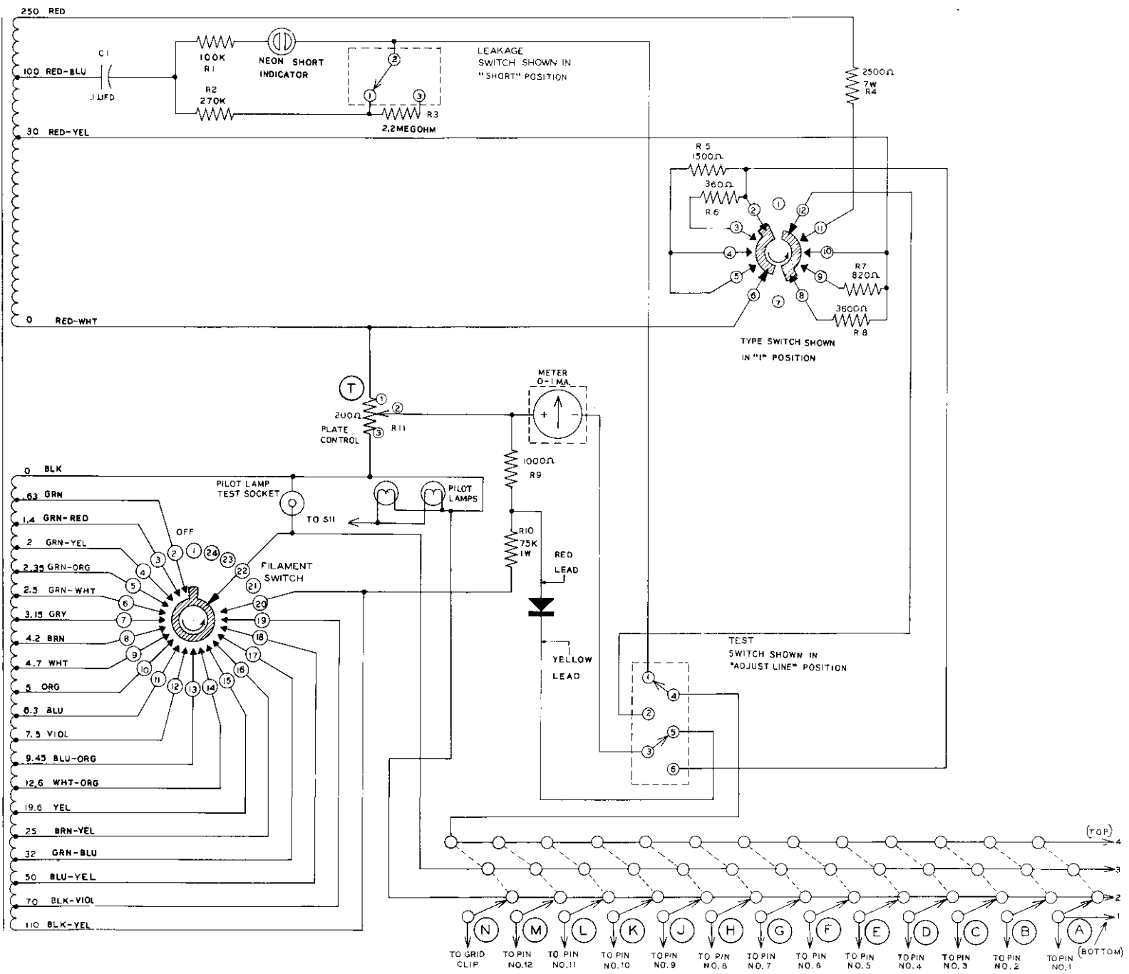
SCHEMATIC OF THE HEATHKIT MODEL IT-21
