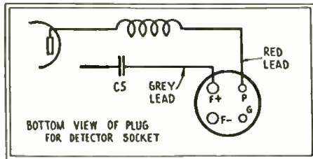
Detail of the plug used to connect the adapter-receiver to the amplifier of a broadcast set, by Fahnestock clips to C5 and the plate choke L4.
