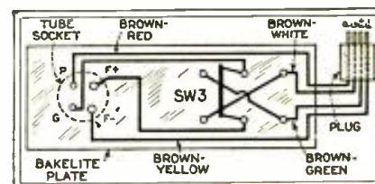
(Q. 44) A Service Man's adapter, to test polarity of dynamic-speaker field connections (see page 373)
