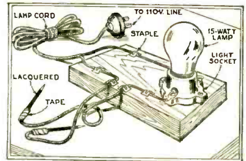
While the cheap, convenient tester pictured is known to many service men, there are others who will find it a useful addition to the kit.
