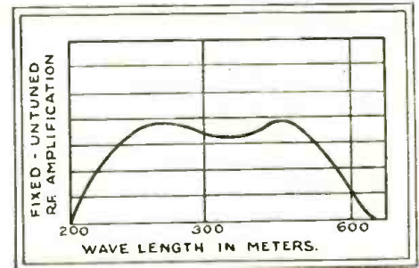
Fig. 1 The old fixed R.F. transformer circuits were fair in the middle of the broadcast band, and poor on the ends.
