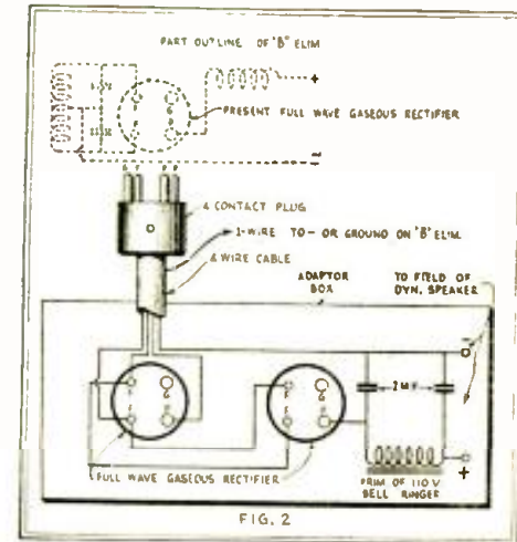
If the power pack of the receiver employs a full-wave, gaseous tube rectifier, the circuit of Fig. 1 is modified in this manner. In this case, the 0.1-mf. "buffer condensers" of the pack are utilized.
