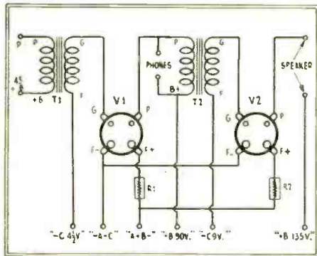
With a '12A output tube, this separate amplifier works a loud speaker nicely. Many short-wave fans will find this more convenient than the use of an adoster with their regular broadcast set.
