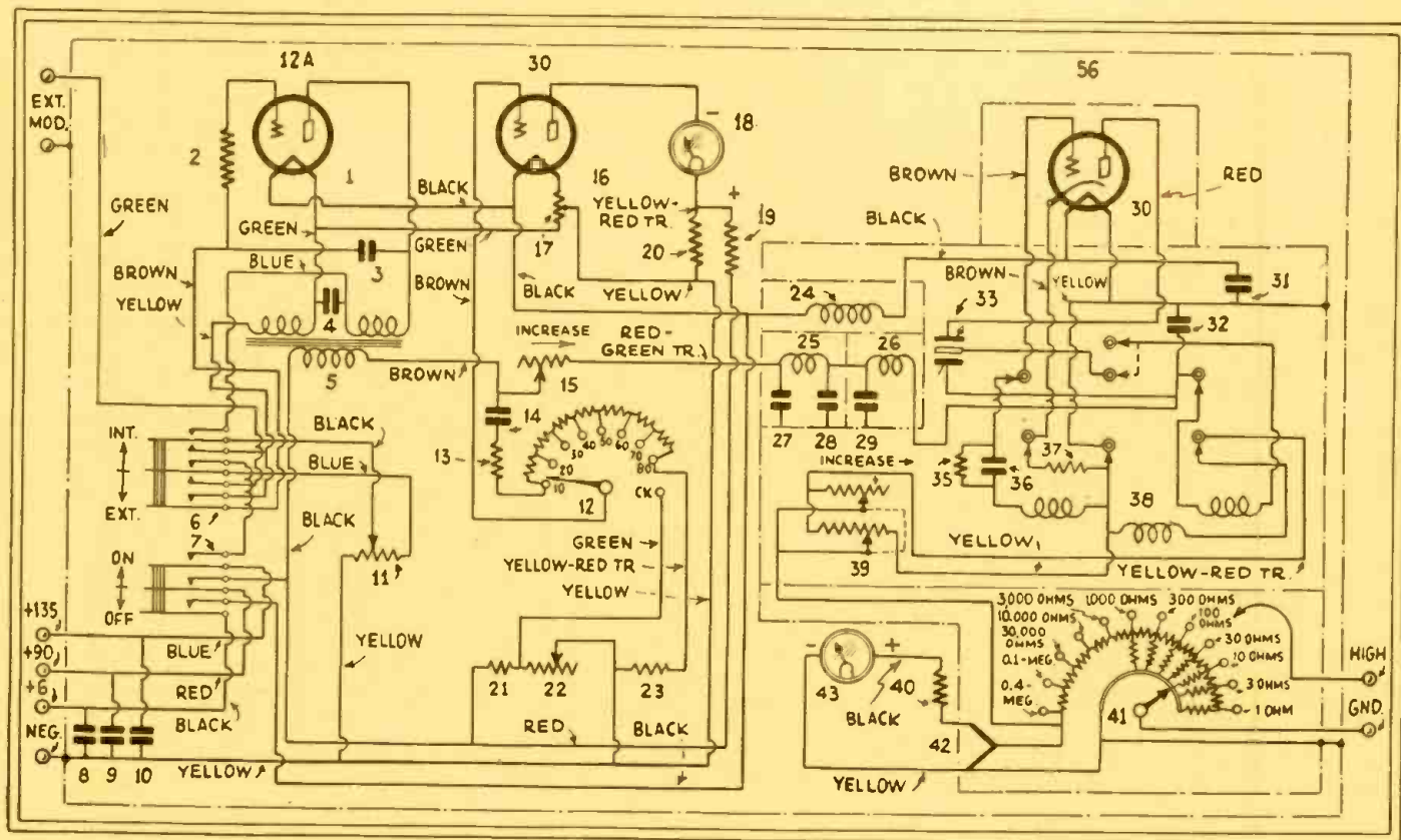
Fig. Q. 197 Complete schematic circuit of the Model TMV-18-C oscillator having a range from 90 to 10,000 kc. Use this on your midget receiver!
