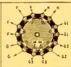
Fig. 2 The special switch used.
