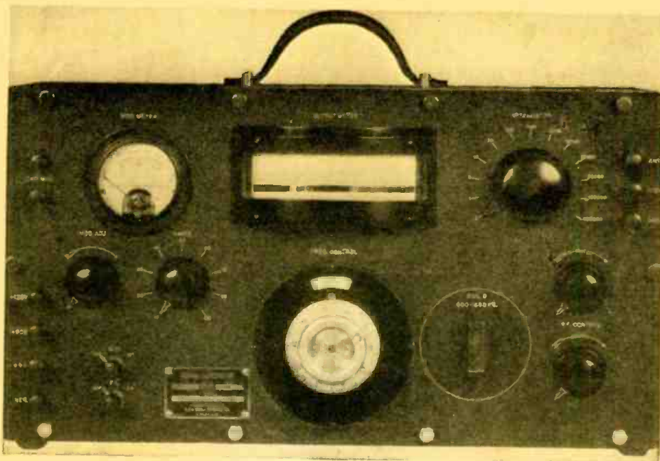
Fig. Q. 197A Photograph of the RCA Victor A.F. modulated R.F. oscillator.
