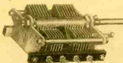
Left, Cardwell transmitting condenser; right, new "Midway" unit.
