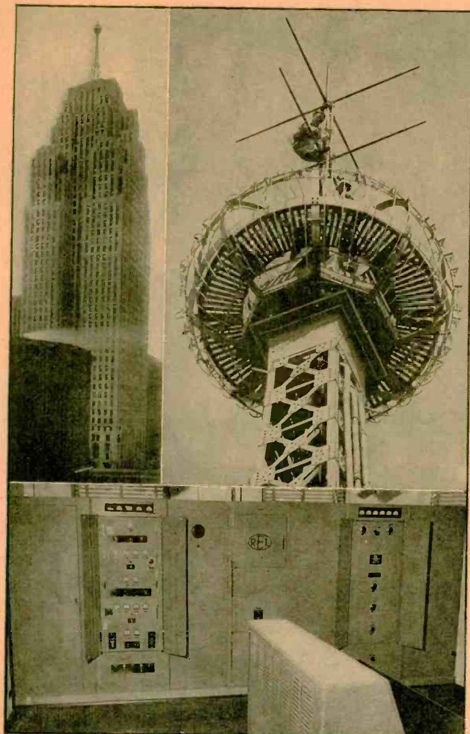
Top left—Station W45D occupies the entire 45th floor of the Penobscot building in downtown Detroit. Top right—2-Bay turnstile antenna atop neon ball and tower. Bottom—R.E.L. 3 KW. driver for 50 KW. amplifier.
