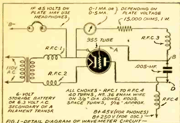
FIG. 1 - DETAIL DIAGRAM OF WAVEMETER CIRCUIT
