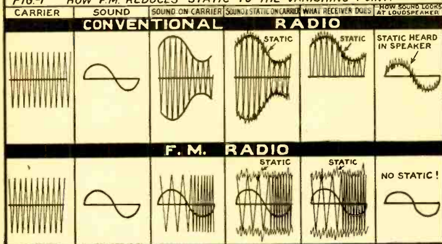
FIG.-1 HOW F.M. REDUCES STATIC TO THE VANISHING POINT.
