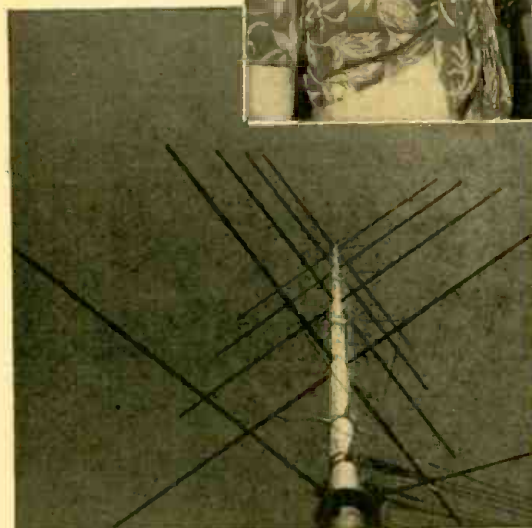
Below — A "bug's-eye" view of the 4-bay turnstile antenna of FM station K45LA. Lower right photo shows the W.E. 1000 watt FM transmitter; note the "blackout" curtains.
