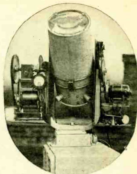
A close-up of the actual pick-up apparatus.
