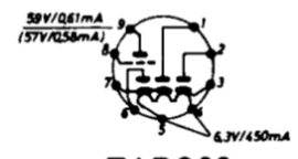
EABC80
