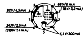
ECH 81
