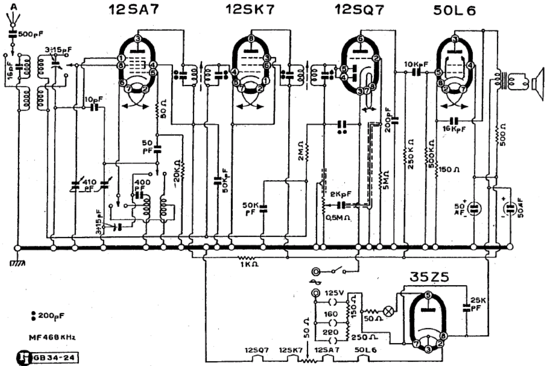
RADIO SUPERLA - Mod. 538
