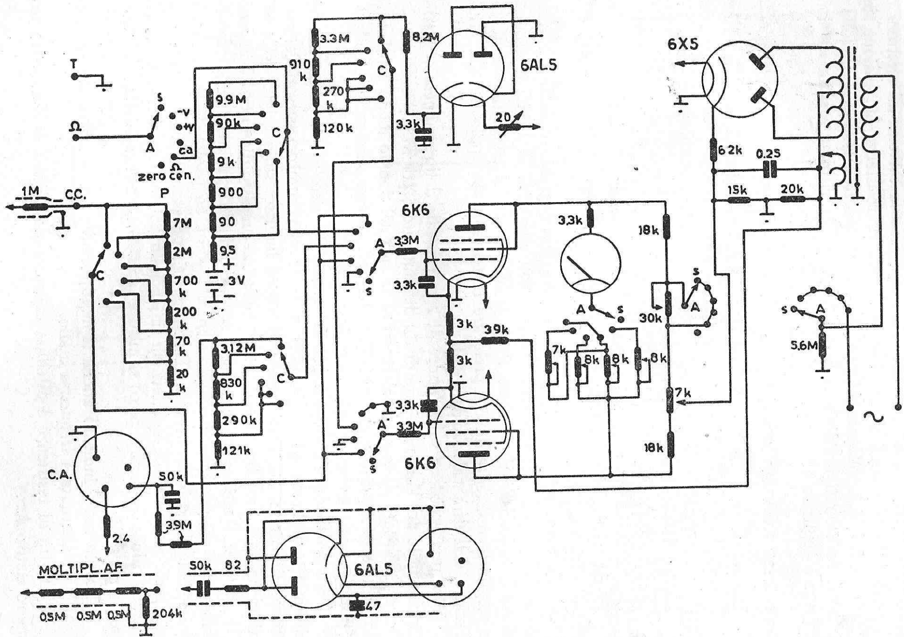
Fig. 66. - Voltmyst RCA Advanced.
