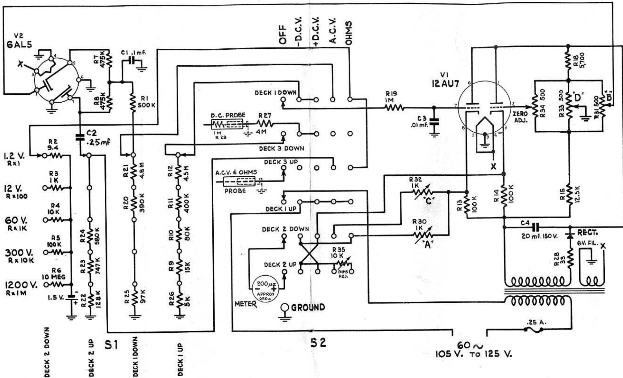
Figure 2 Model 303 Schematic Diagram
