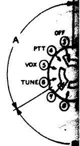
FUNCTION SWITCH (REAR VIEW)
