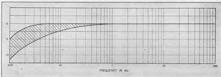
Frequency characteristic of the multiplier.
