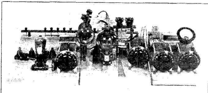
AT THE LEFT IS THE LAST FREQUENCY DOUBLER, A UX-210. This shows somewhat more clearly the input circuit to the pair of 252's and the two neutralizing condensers. The breadboard on the right holds the antenna tuning equipment as well as the meter.
