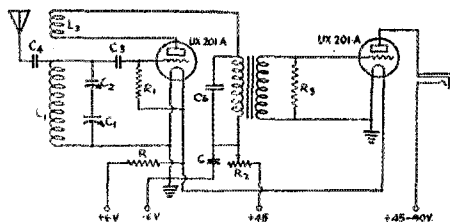
FIG. 4. THE SIMPLE WIRING OF THE TWO-TUBE SET
