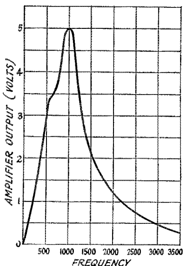
FIG. 1. A CURVE OF FREQUENCY VS. OUTPUT VOLTS TAKEN WITH THE THREE-TUBE RECEIVER
