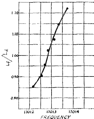
FIGURE 3. THE RATIO OF THE CHANGE OF INDUCTANCE PLOTTED AGAINST FREQUENCY.
