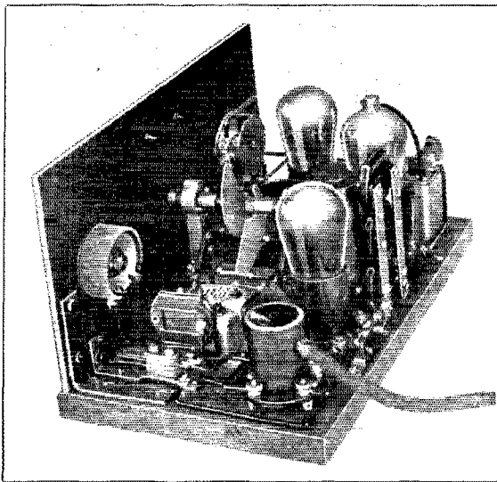
ANOTHER VIEW OF THE THREE-TUBE RECEIVER
