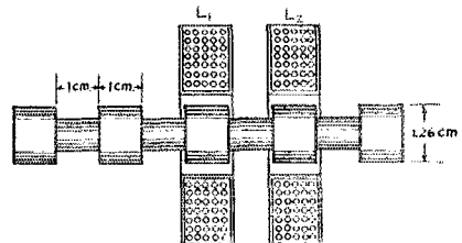
FIGURE 4. THE ROD CONSISTS OF FIVE BEADS CONNECTED BY SECTIONS OF HALF THEIR DIAMETER. All sections are of equal width. This rod vibrates at 295,130 cycles per second. The rod may also be made to vibrate with one of the beads between the two coils and the thinner sections within the coils.
