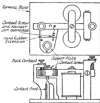
FIG. 3 KEYING RELAY
