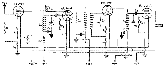
FIG. 2. THE WIRING OF THE FOUR-TUBE RECEIVER
