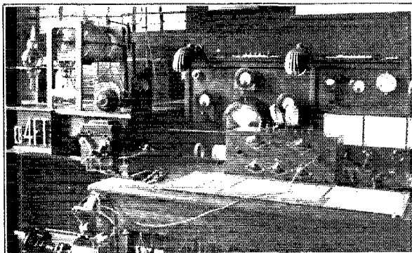
AMATEUR STATION #64FT, OWNED AND OPERATED BY GEORGE NEELEMANS. TRAFFIC MANAGER OF THE RESEAU BELGA AT BRUSSELS, BELGIUM, is one of the most widely known amateur stations in the world. The circuits is a Meeny, with two 150-watt Mullard valves. An Esco motor generator supplies 1100 volts for them. The antenna is a half-wave Zeppelin working on 32 meters. All instruments are Westons, and the receiver is a Grebe CR-18. These, with the Esco m. g. and the Vibronlex key c64FT, to use the words of its owner "rather a Yank station in appearance!"
