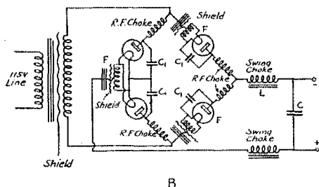
FIG. 4B — SINGLE-PHASE BRIDGE-TYPE RECTIFIER PROTECTED FOR TUNABLE HUM
