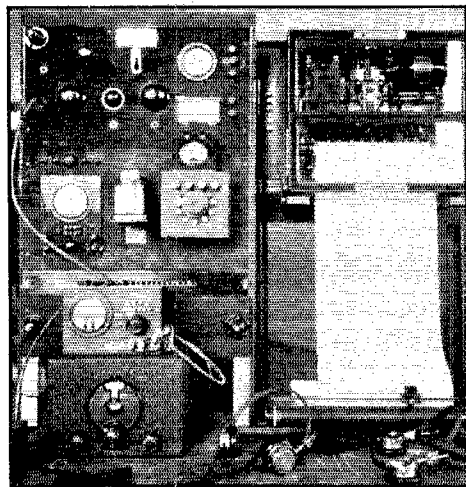
EQUIPMENT USED AT THE CASE SCHOOL OF APPLIED SCIENCE, CLEVELAND, FOR GRAPHICAL RECORDING OF THE SIGNALS OF WIEKL
