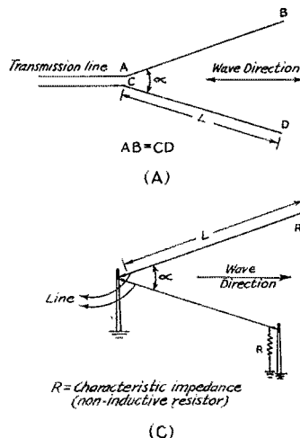
FIG. 3—(A) THE "V" ANTENNA; (C) "V" ANTENNA TERMINATED TO ABSORB BACK RADIATION AND THUS PRODUCE A UNIDIRECTIONAL PATTERN
