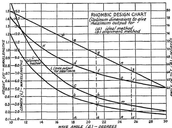
FIG. 6—RHOMBIC ANTENNA DESIGN CHART
