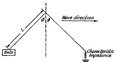
FIG. 2-A—TILTED-WIRE ANTENNA OR "INVERTED V"
