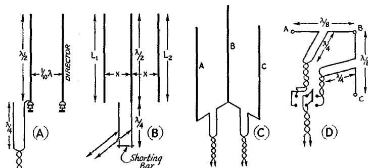
Fig. 6 — Simple directive systems using vertical elements.
