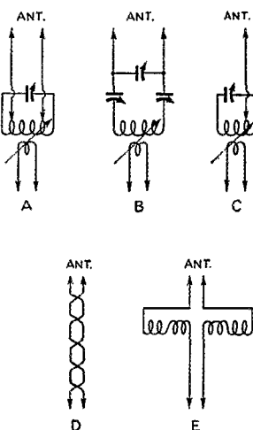
Fig. 1—Antenna coupling systems. A—For medium impedance transmission lines. B—For tuned lines. C—For voltage-fed antennas or single-wire transmission lines. D—Low-impedance line. E—Variable-inductance coupler.
