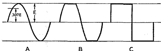
Fig. 2—Three types of waves having the same peak values but containing different amounts of power. A, the familiar sine wave; B, flat-topped wave typical of an overdriven Class-B stage; C, the extreme case of a square wave.
