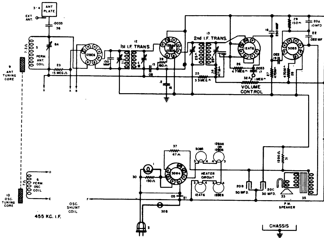
SCHEMATIC DIAGRAM—MODEL 56TG-M, 56TH-M, 56TJ-M (MINIATURE)
