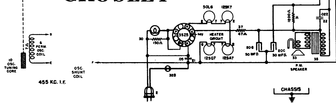
SCHMATIC DIAGRAM—MODEL 56TG-O, 56TH-O, 56TJ-O (OCTAL)
