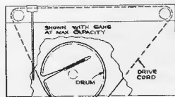
Dial Cord Assembly
