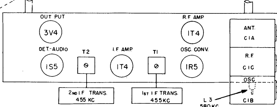
Tube and Trimmer Location (Model 165)
