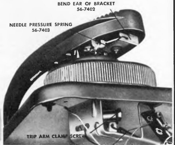
FIGURE 9. NEEDLE-PRESSURE ADJUSTMENT
