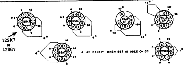
VOLTAGE TABLE (BOTTOM VIEW OF CHASSIS)
