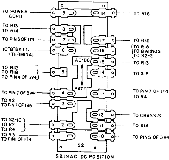
Switch Connections
