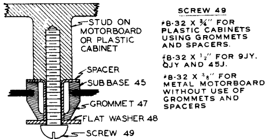
Figure 25—Sub-base Mounting.
