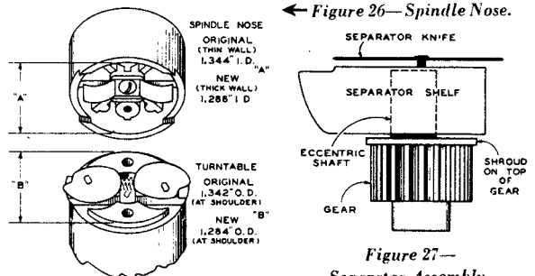
Figure 26—Spindle Nose.
