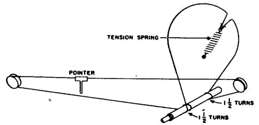
DIAL DRIVE
