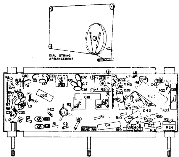
LOCATION OF PARTS AND TRIMMERS UNDER CHASSIS
