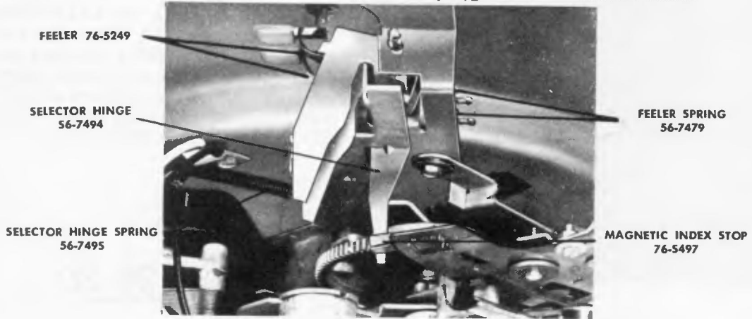
FIGURE 1. 7" INDEX ADJUSTMENT
