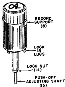
Figure 7. 45 RPM Centerpost.
