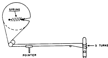
DIAL DRIVE
