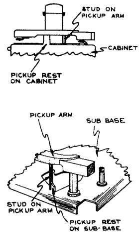
Figure 24—Pickup Arm Rest.
