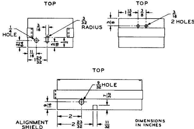
Fig. 3—Alignment Shield
