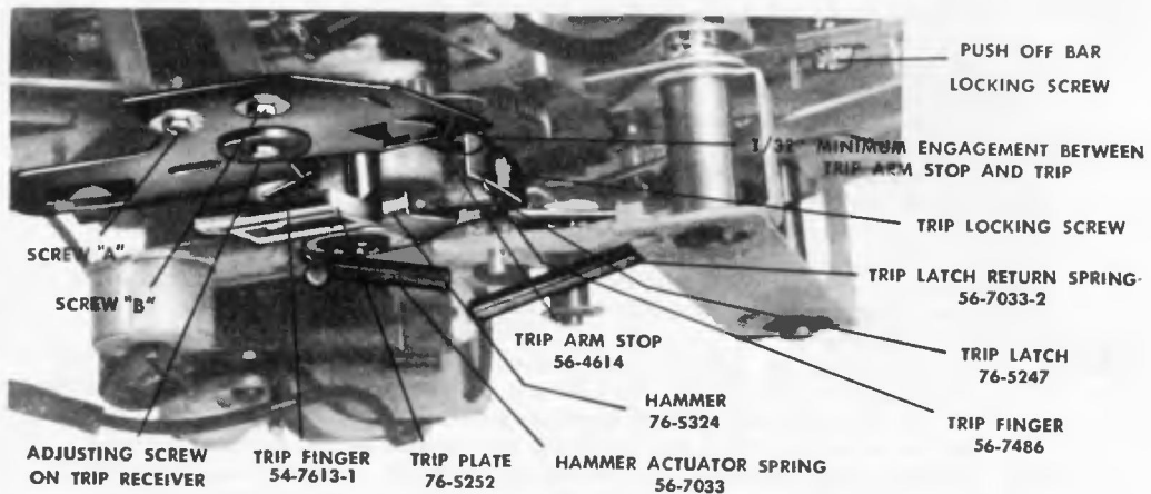
FIGURE 3. TRIP ADJUSTMENTS
