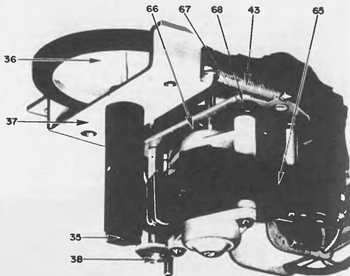
Spindle S-17424
