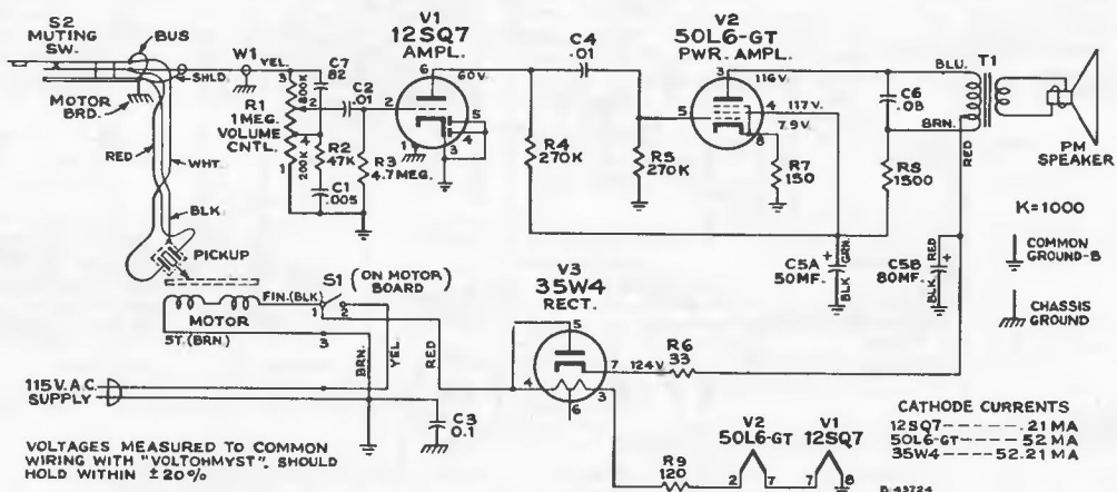
Schematic Diagram RS138A
