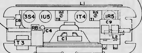
TUBE LAYOUT
