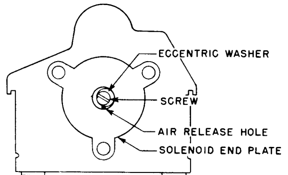
FIGURE 3. AIR RELEASE ADJUSTMENT
