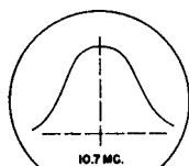
ALIGNMENT CURVES (FM)
