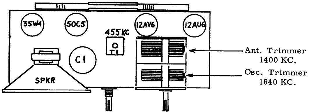
Chassis Top View
