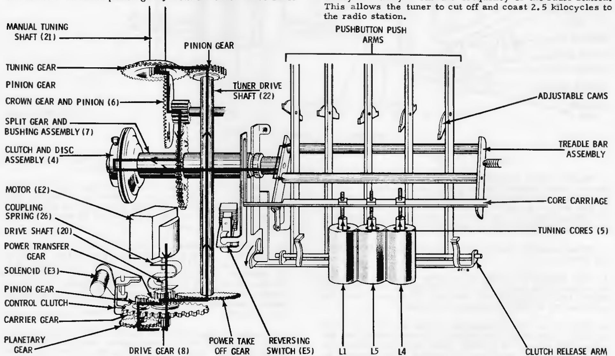
FIGURE 6. SEARCH TUNING
