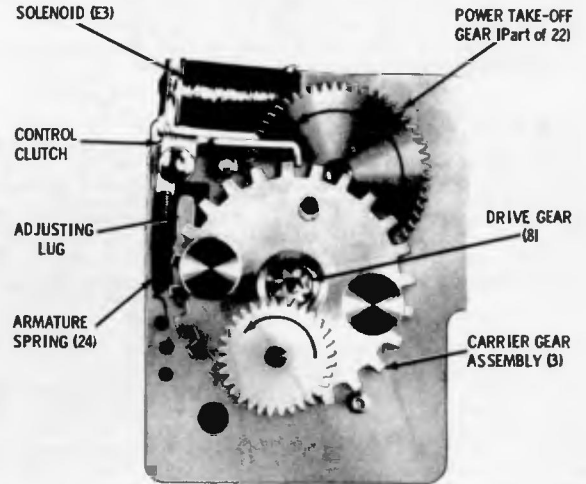
FIGURE 10. CLUTCH ENGAGED
