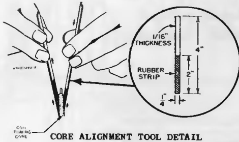
CORE ALIGNMENT TOOL DETAIL
