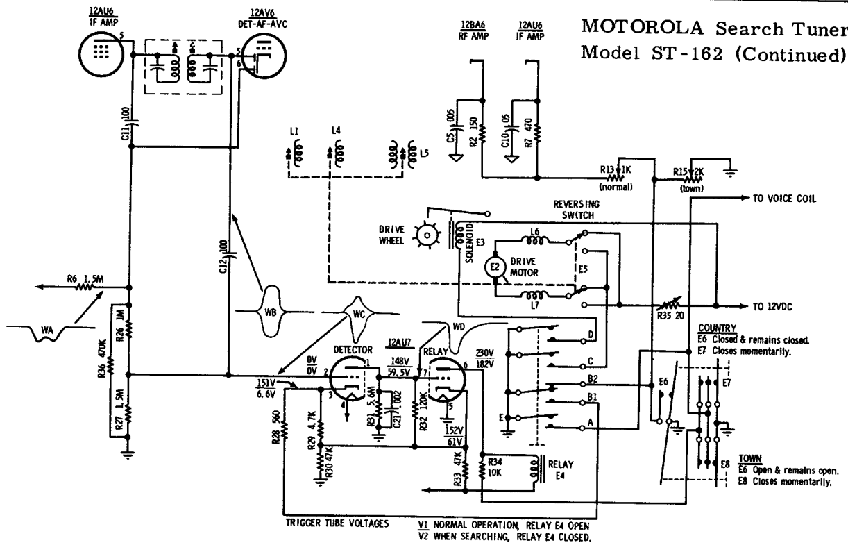
FIGURE 7. FUNCTIONAL SCHEMATIC
