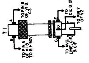
R-F Coil Wiring
