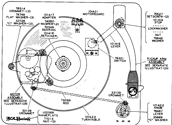
Motorboard Assembly
