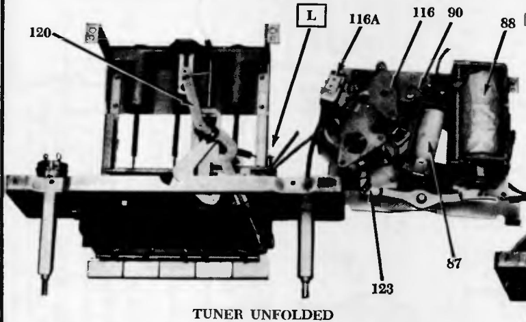
TUNER UNFOLDED
