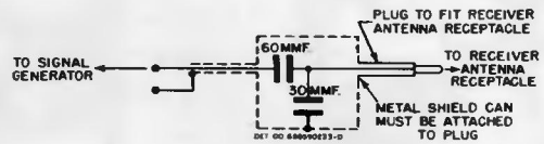
DUMM ANTENNA DETAIL
