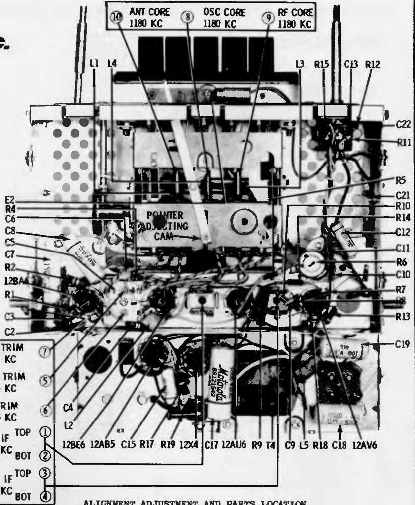
ALIGNMENT ADJUSTMENT AND PARTS LOCATION
