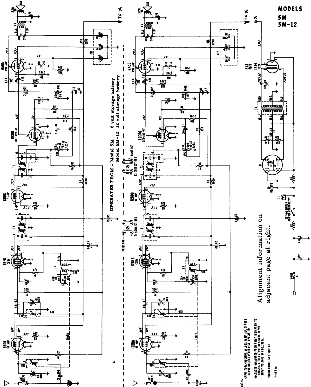
MODEL 5M SCHEMATIC DIAGRAM
