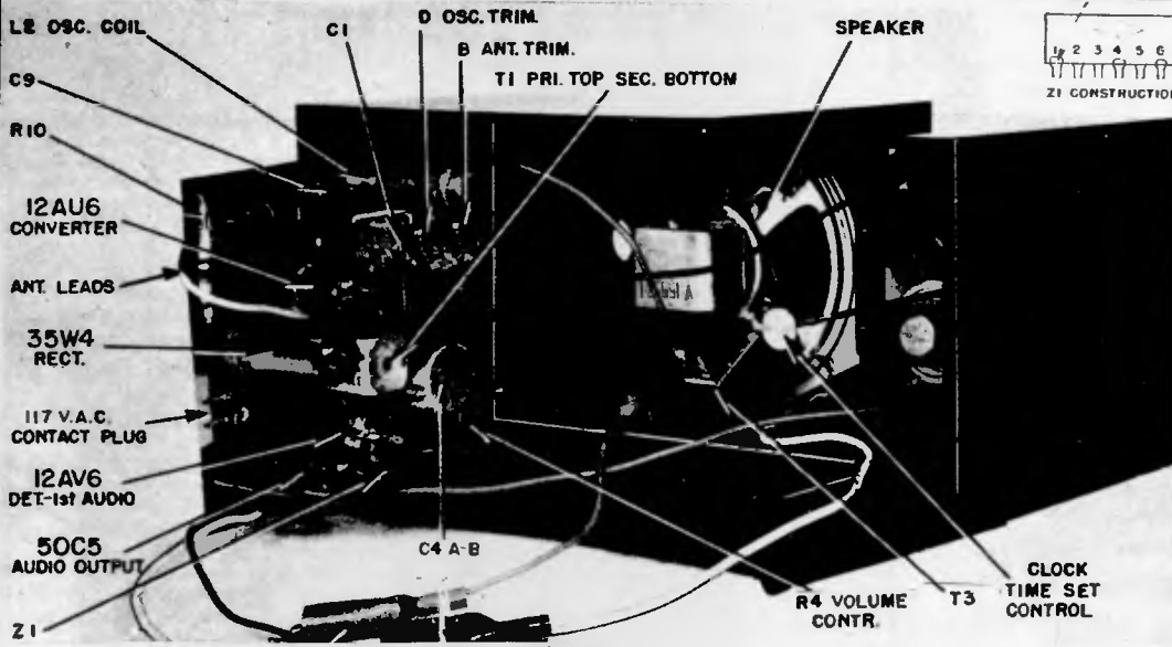
ALIGNMENT
