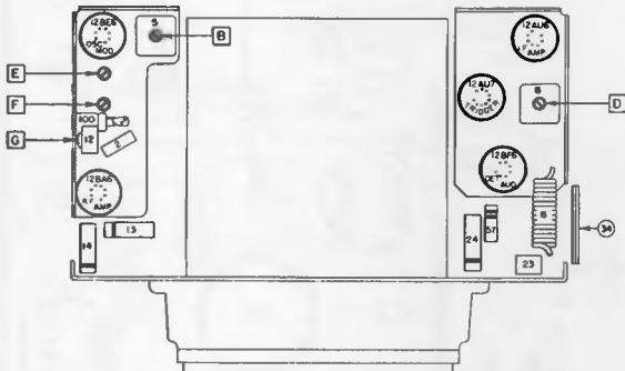
PARTS LAYOUT — TUBE VIEW
