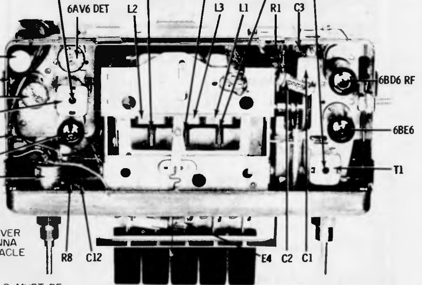
PARTS LOCATIONS & ALIGNMENT ADJUSTMENTS
