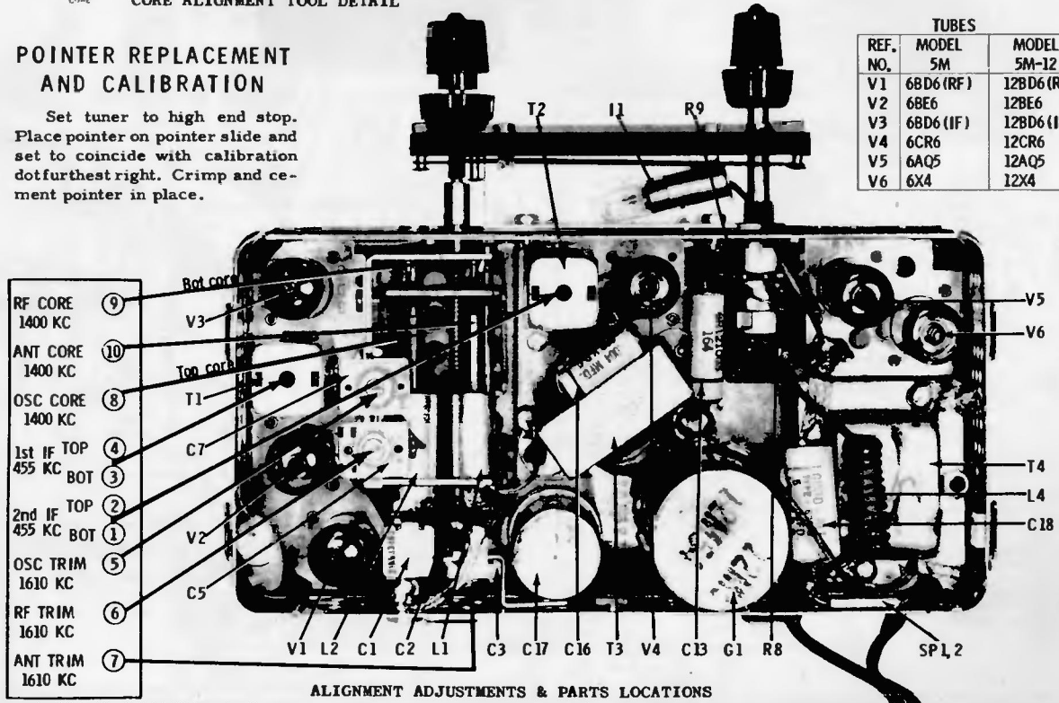
ALIGNMENT ADJUSTMENTS & PARTS LOCATIONS
