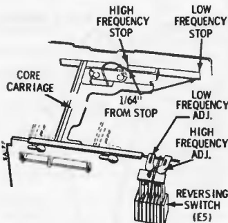
FIGURE 12. REVERSING SWITCH ADJUSTMENT
