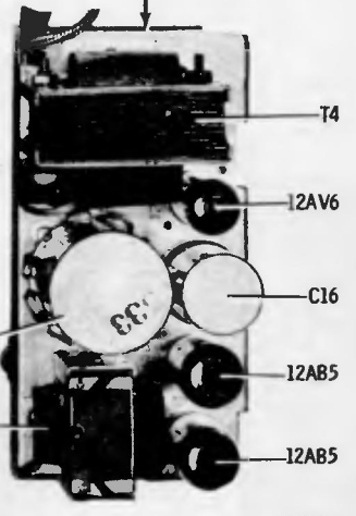
TOP VIEW POWER SUPPLY 841, 842 & 843
