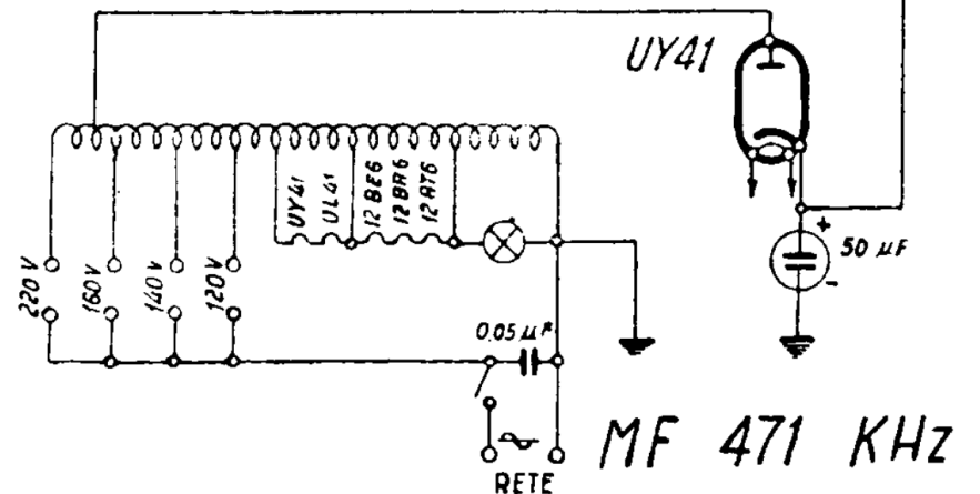
MAGNADYNE RADIO - Mod. S 12, mod. Kennedy K 412 e mod. Damaiter M 812. Gamme onde medie. Media frequenza 471 kc/s.
