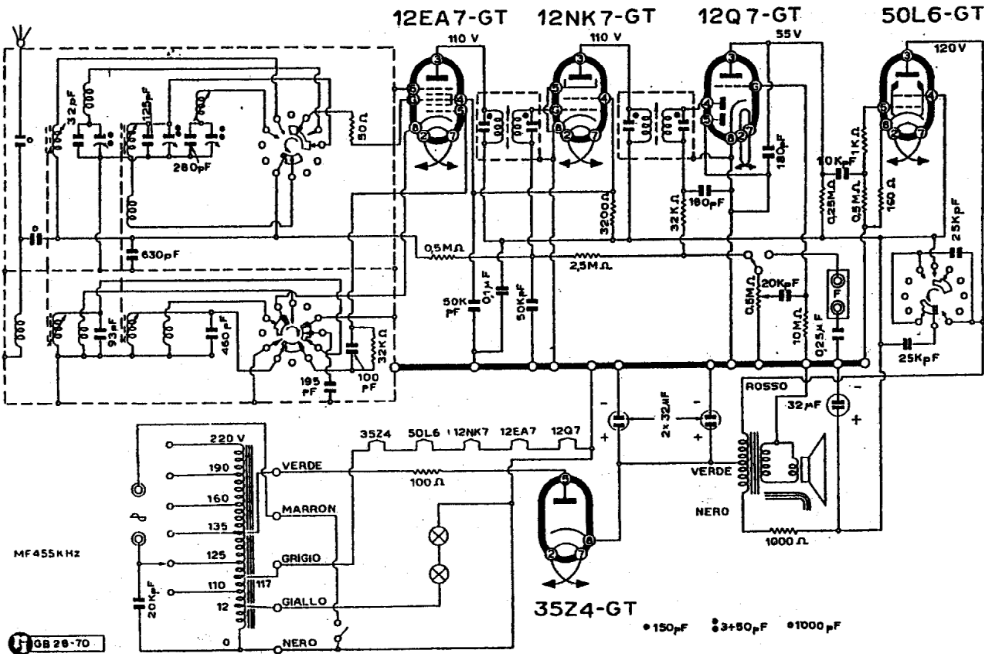
Radiomarelli 10A151M
