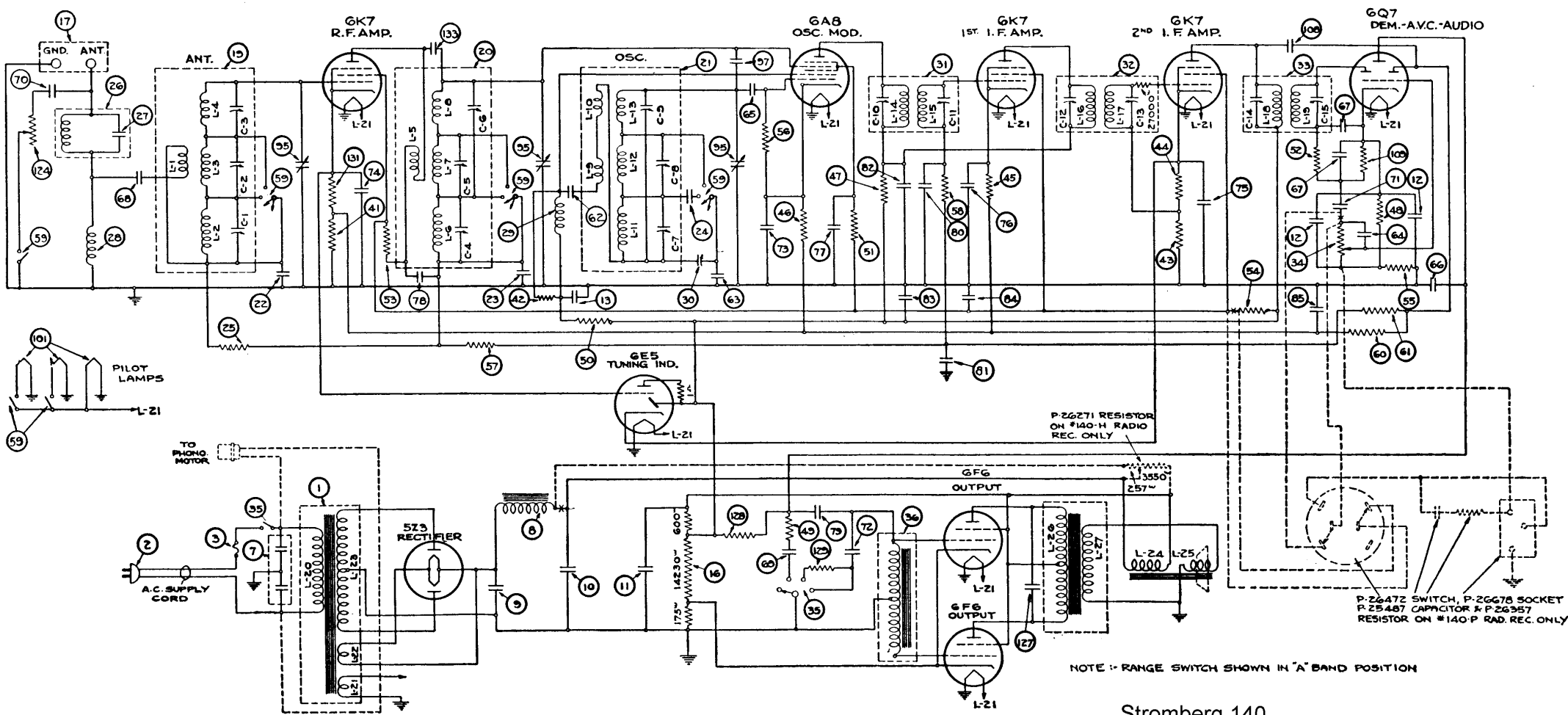
Fig. 3. Schematic Circuit of Receiver.
