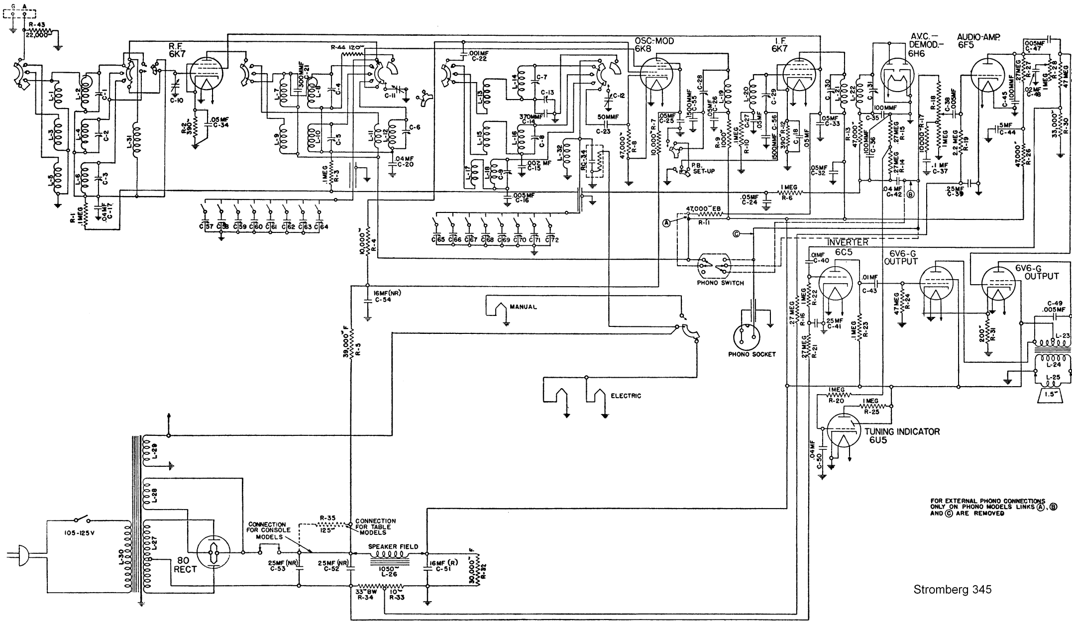
Fig. 2. Schematic Circuit of Receiver.
