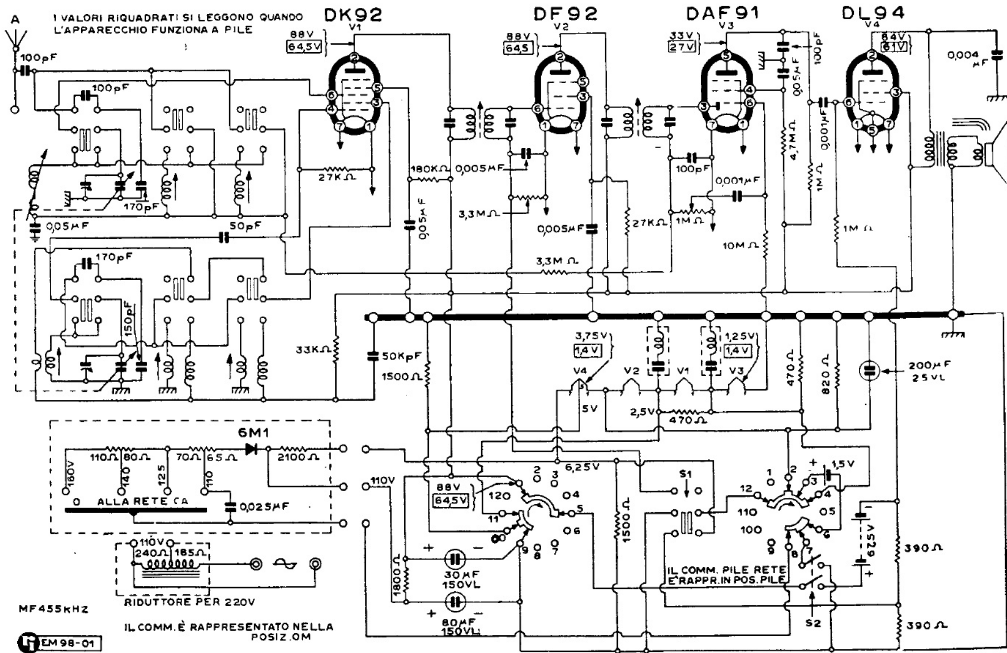
F.A.R.E.T. - Mod. Personal 503 Dinghy
